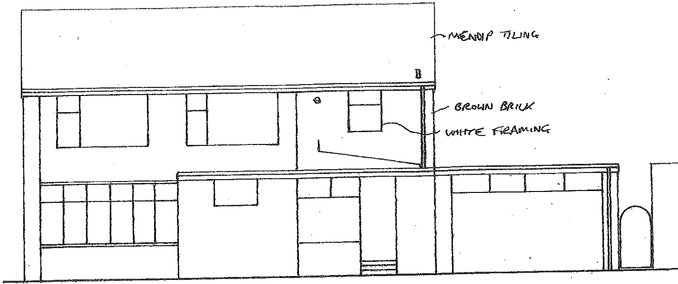
EXISTING FRONTAGE 1:100
